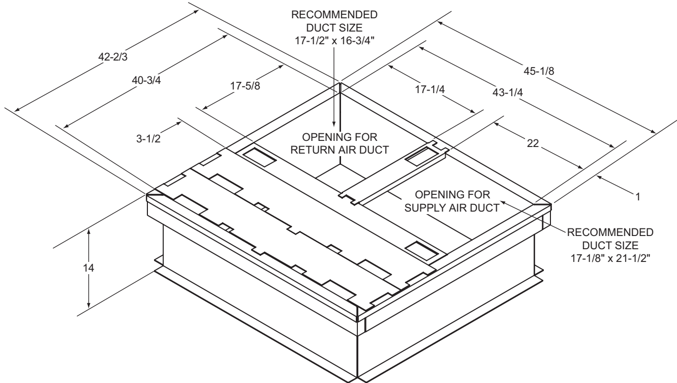
Figure 6: Roof Curb 1
